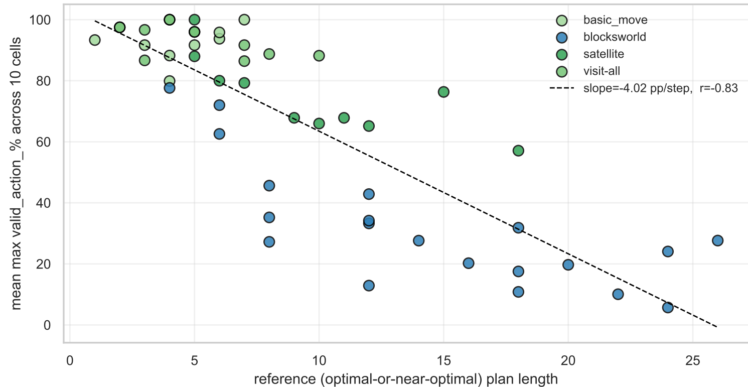
Plot 15 - Reference difficulty vs empirical model performance
