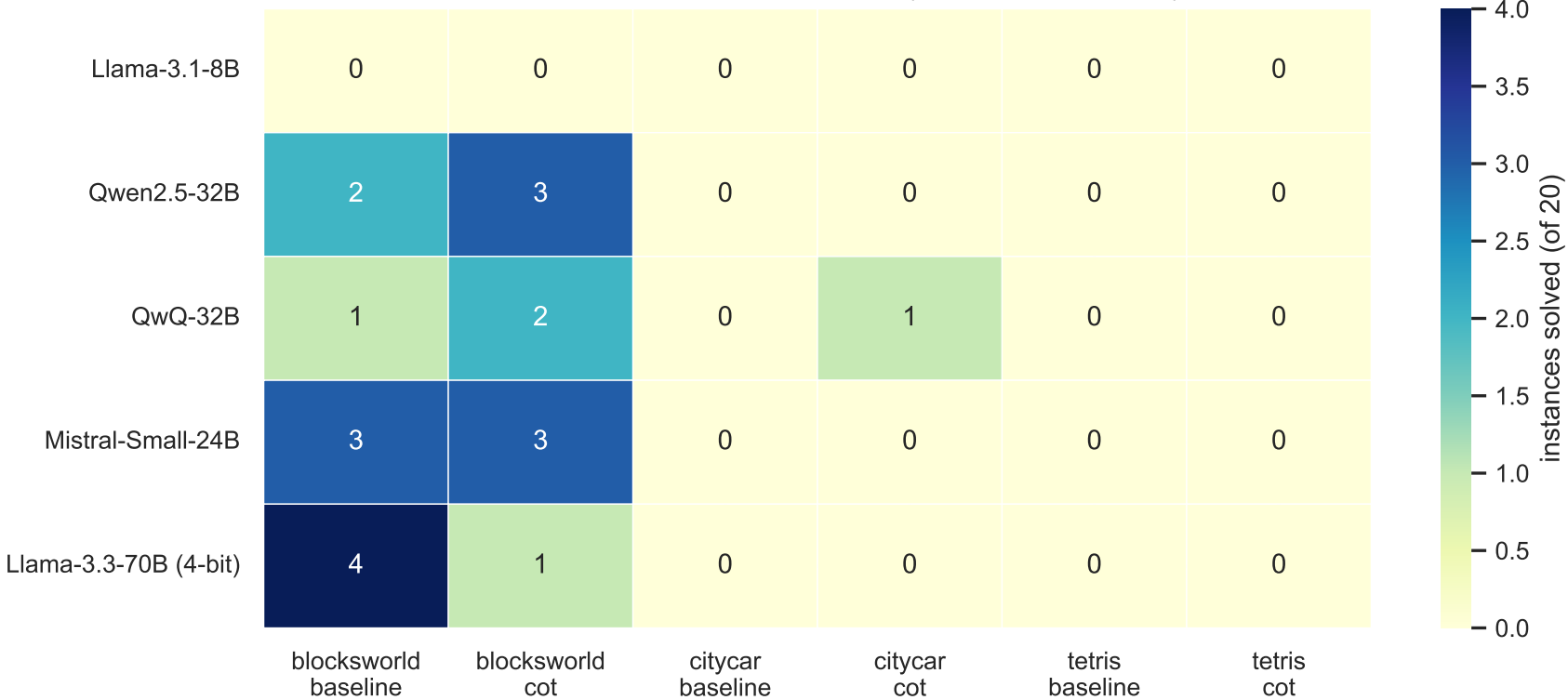
Plot 1 — Full-solve count per cell (success rate matrix)
