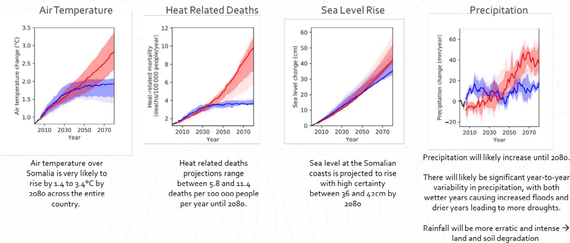
From the Climate Risk Profile: Somalia | Weathering Risk
