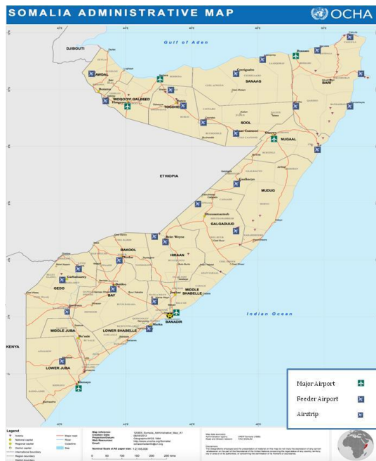
Map3: Major airports and airstrips in Somalia 19
