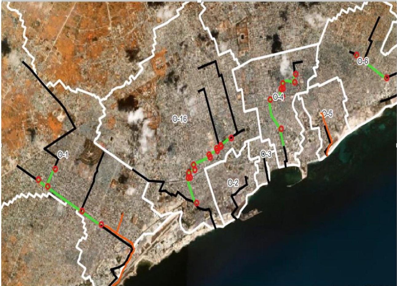
Map of Mogadishu Trunk Drainage Lines (Masterplan Preferred Option 2)
