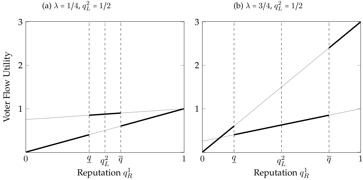
Figure 4: Variation of Voter Flow Utility with \lambda
