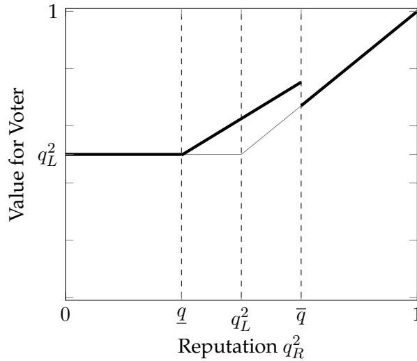
Figure 3: Learning Value of \pi^* for Voter
