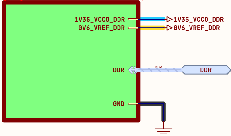
Zynq Bank 502 (PS DDR)
