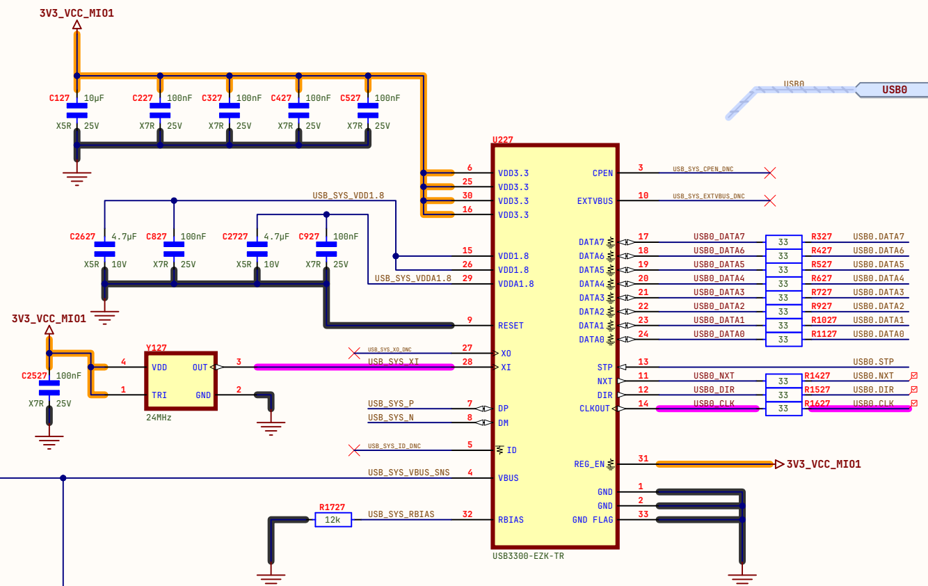
USB CONTROLLER
