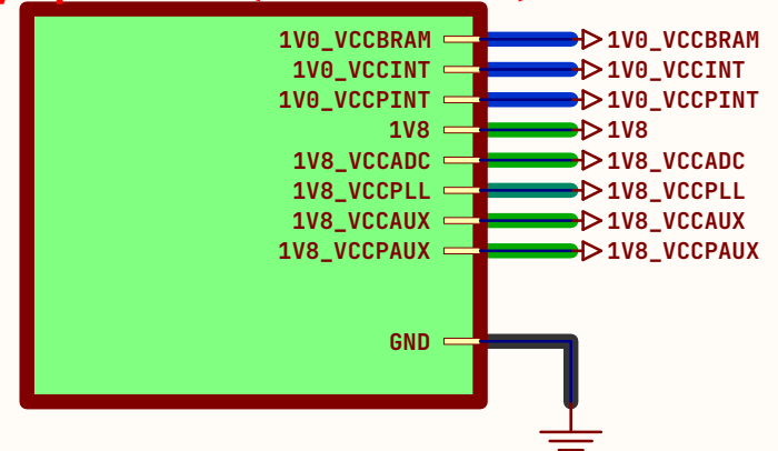
Zynq Power (Core Rails)
