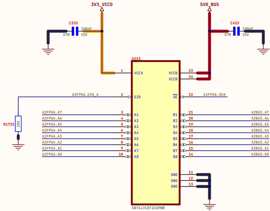
ADDRESS LINES 0..7
