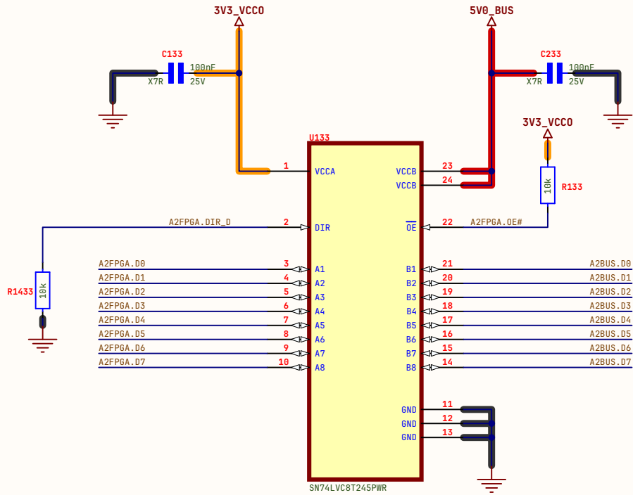
BI-DIRECTIONAL DATA LINES
