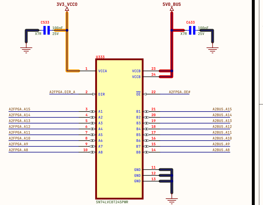
ADDRESS LINES 8..15
