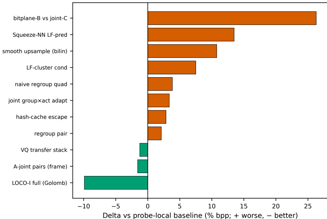
Negative atlas (selected; each bar own baseline)
