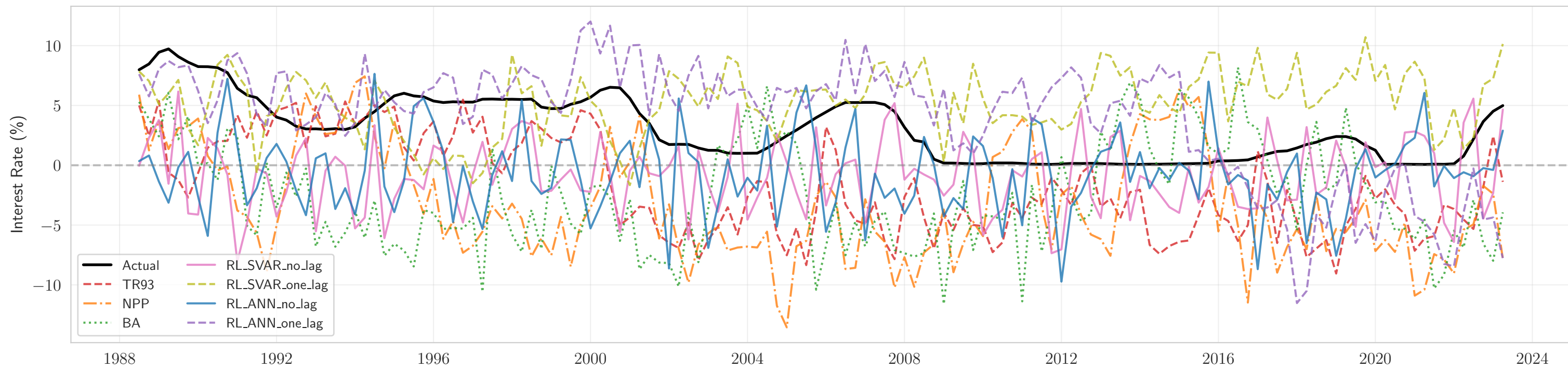
Historical Counterfactual: Linear Policies
