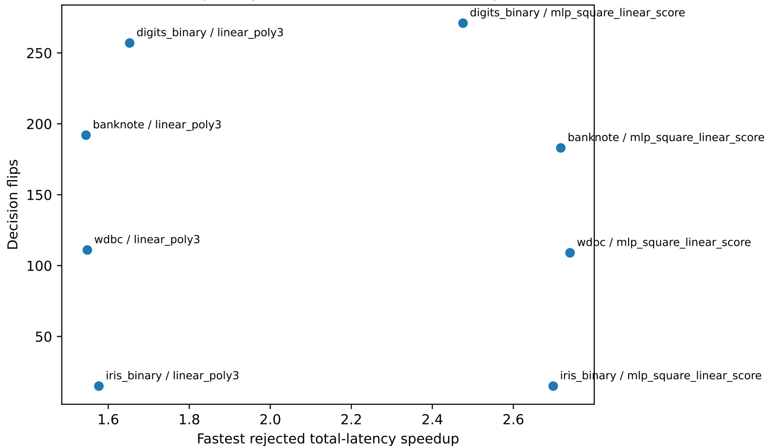
Raw speed gain versus decision instability
