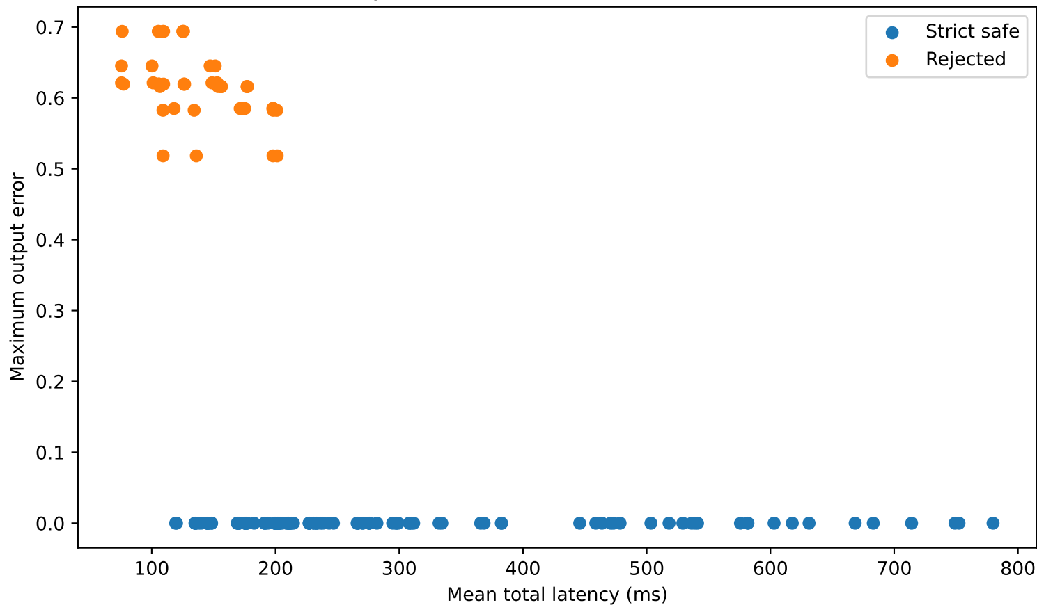
Latency-error tradeoff across CKKS candidates
