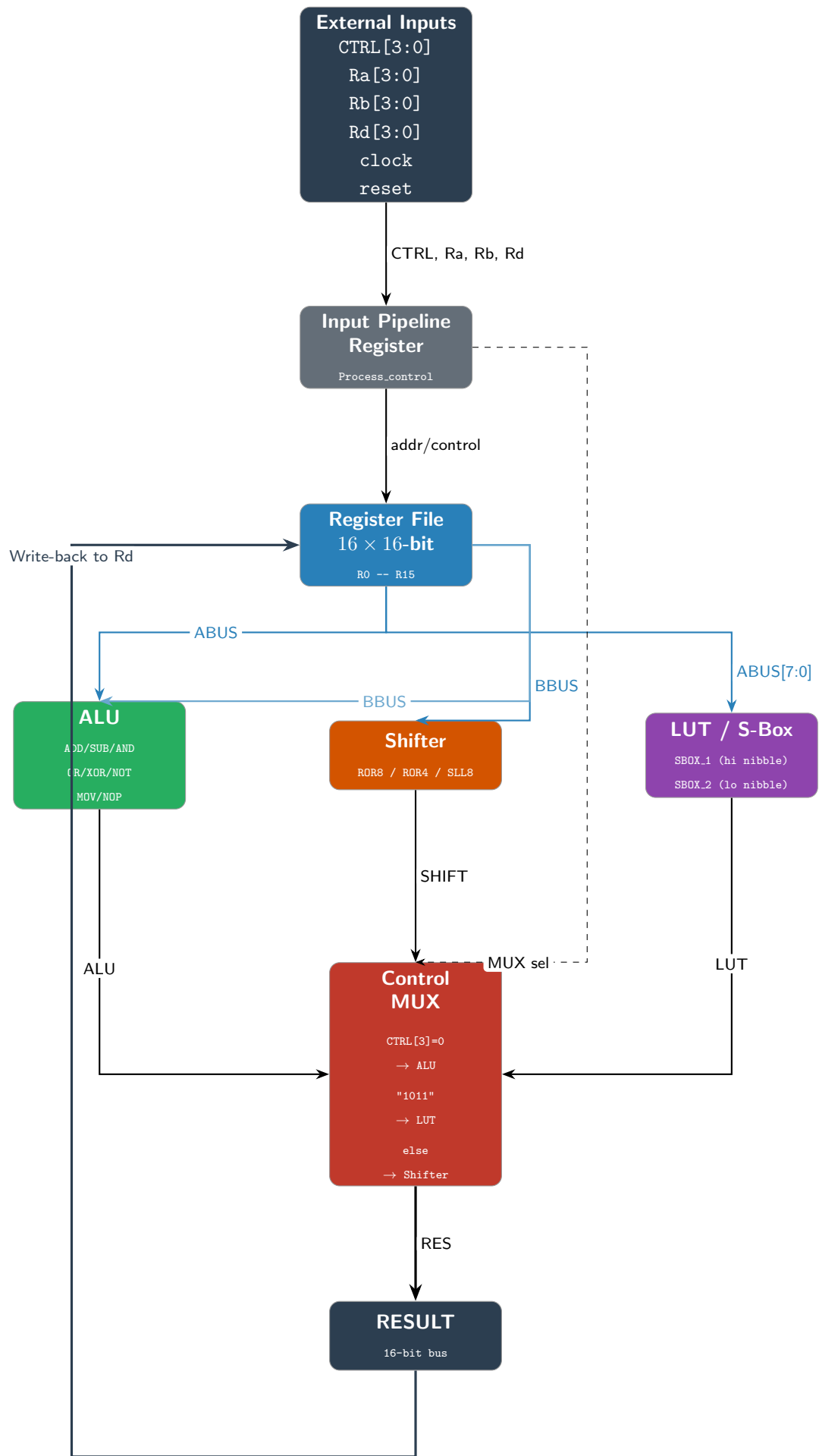
Figure 1: dataflow of CryptoCore-16
