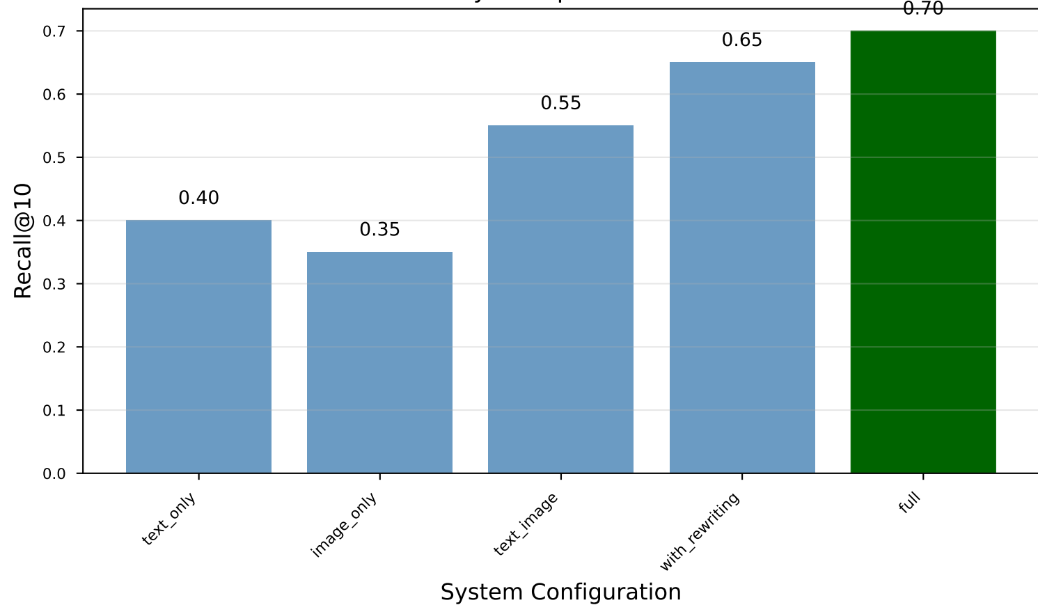
Ablation Study: Component Contributions
