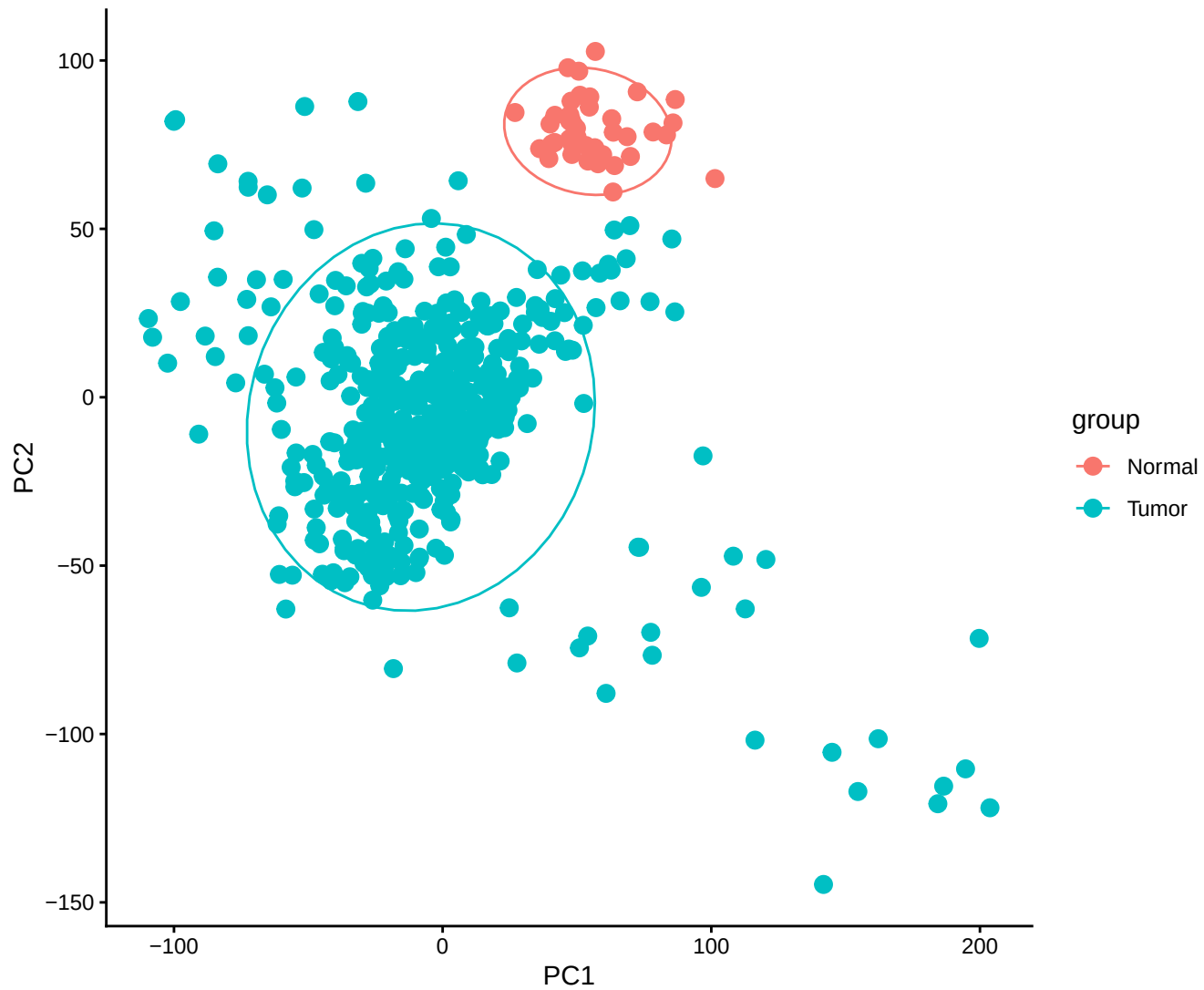
PCA of COAD Tumor vs Normal
