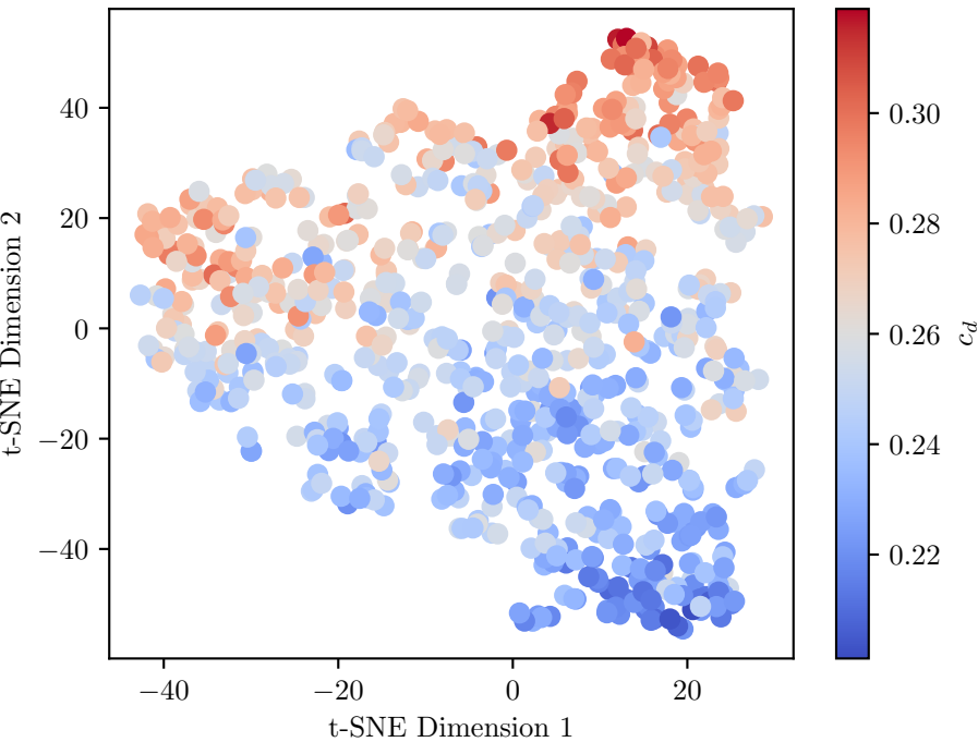
t-SNE Projection of Latent Space
