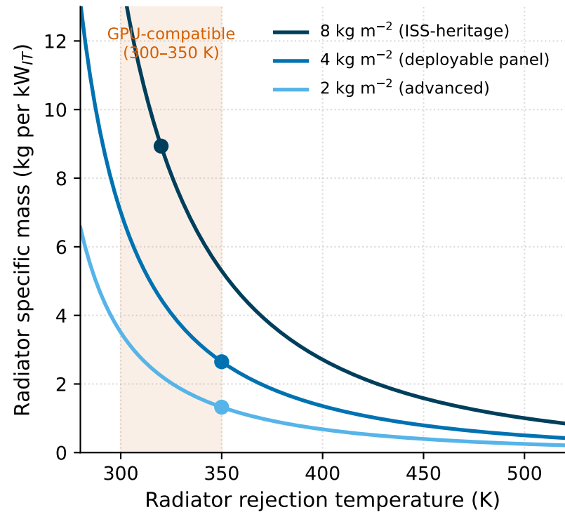
(a) Specific mass vs. temperature (Stefan-Boltzmann)
