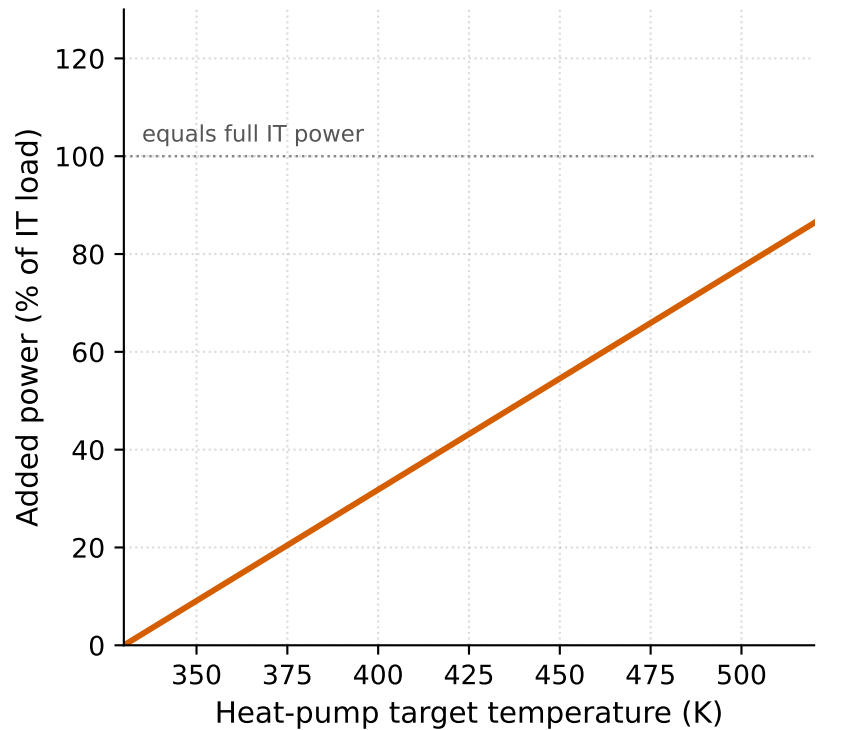
(b) Heat-pump penalty to raise rejection T from 330 K
