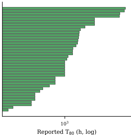
Every T_{80} in six months (n=39)
