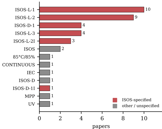
Any stability protocol named: 39 of 872
