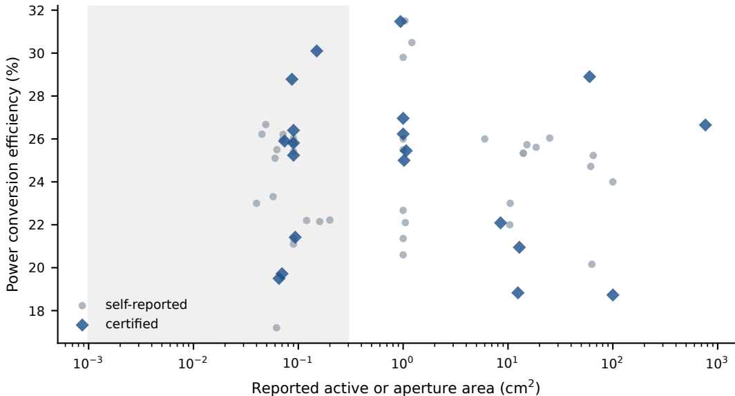
58 papers reporting both an area and an efficiency, spanning 0.04 to 764 cm 2 . Shading marks the sub-0.3 cm 2 laboratory-cell regime.
