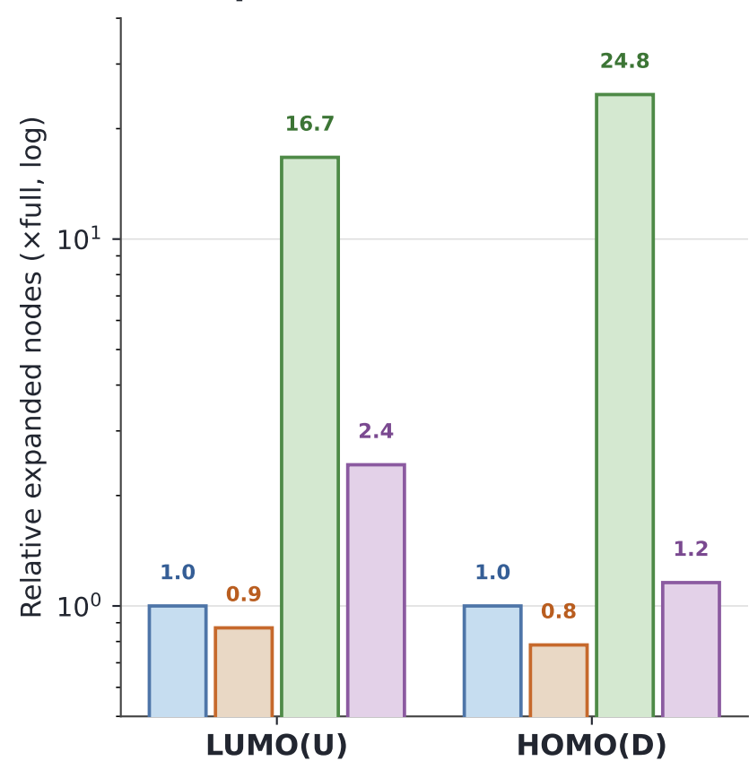
(c) Expanded nodes (fold vs full)
