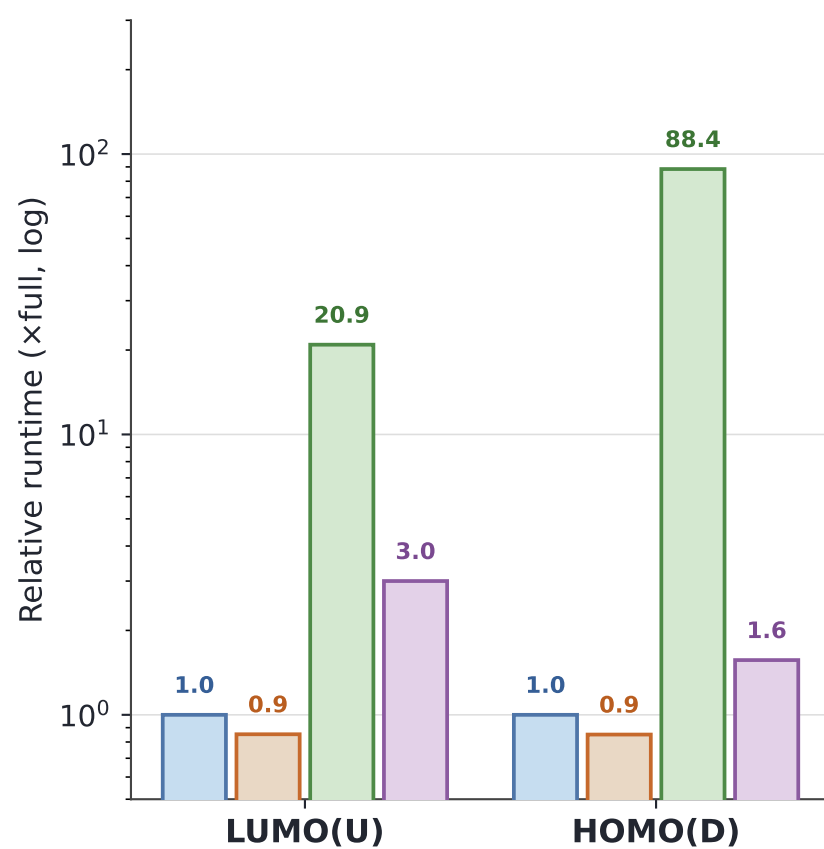
(b) Runtime (fold vs full)
