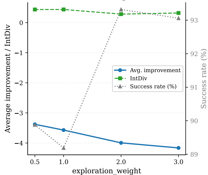
(a) LUMO(D): exploration
