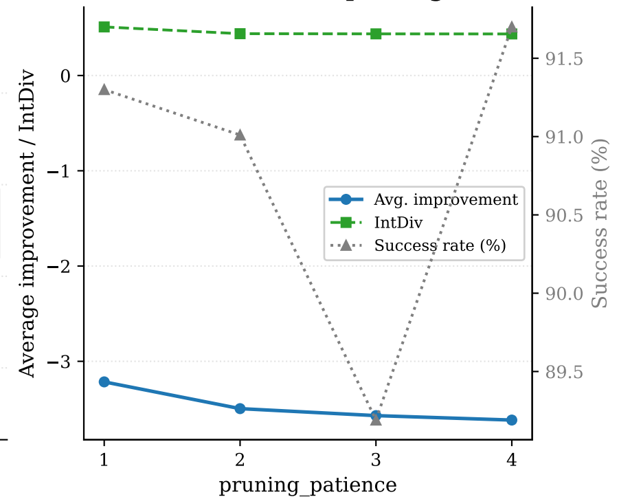
(c) LUMO(D): pruning
