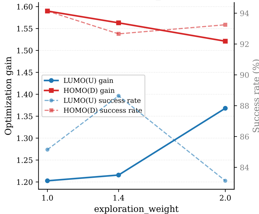
(b) exploration_weight
