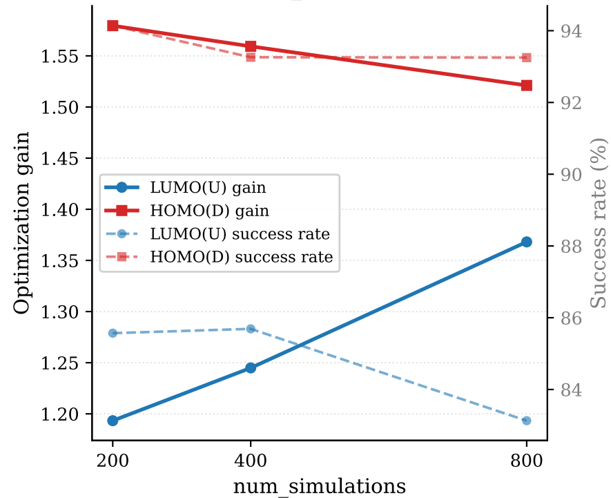
(a) num_simulations
