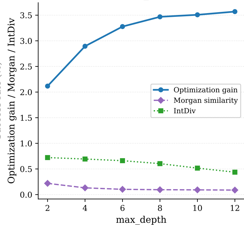
(c) max_depth
