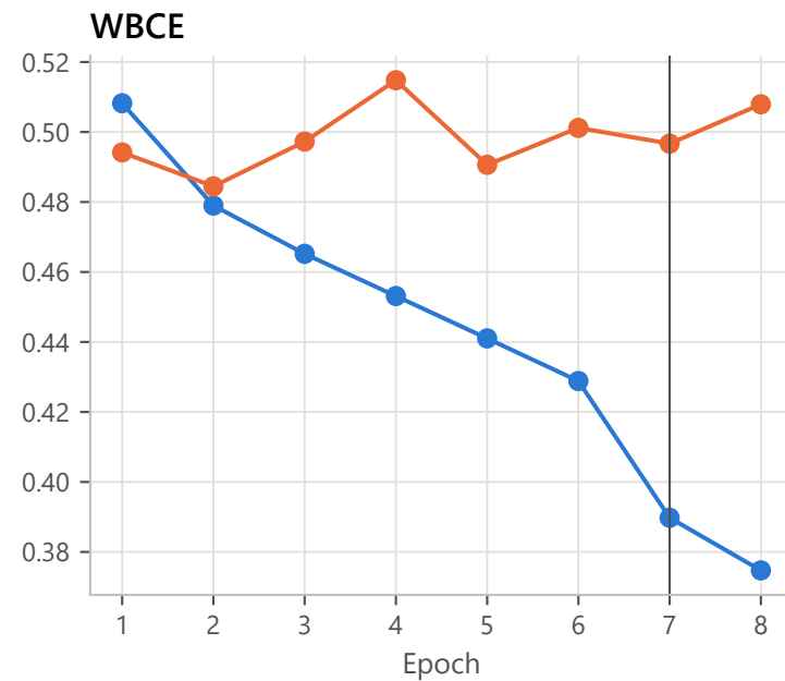
Train vs validation loss per arm (loss scales differ between loss functions; compare shapes only)
