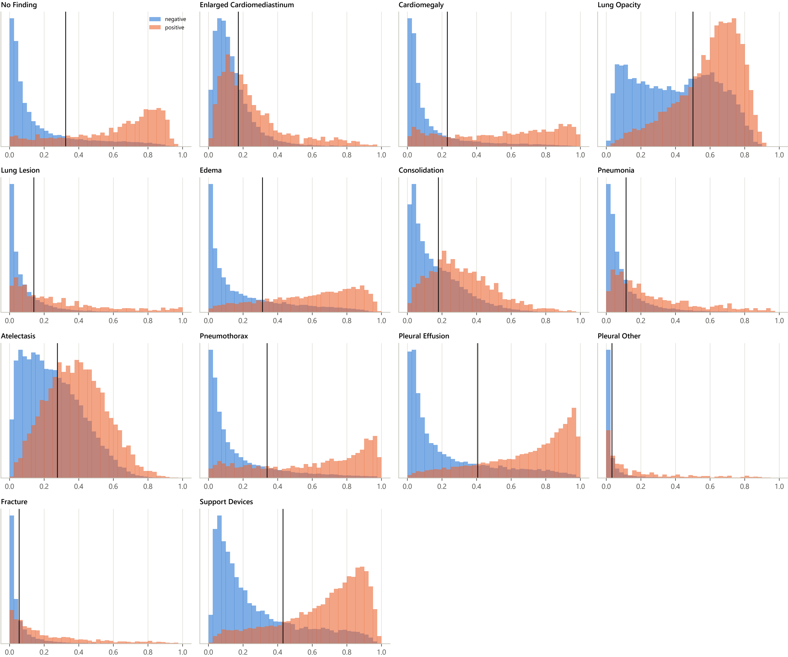
Validation probability distributions by true label (line = Youden threshold)
