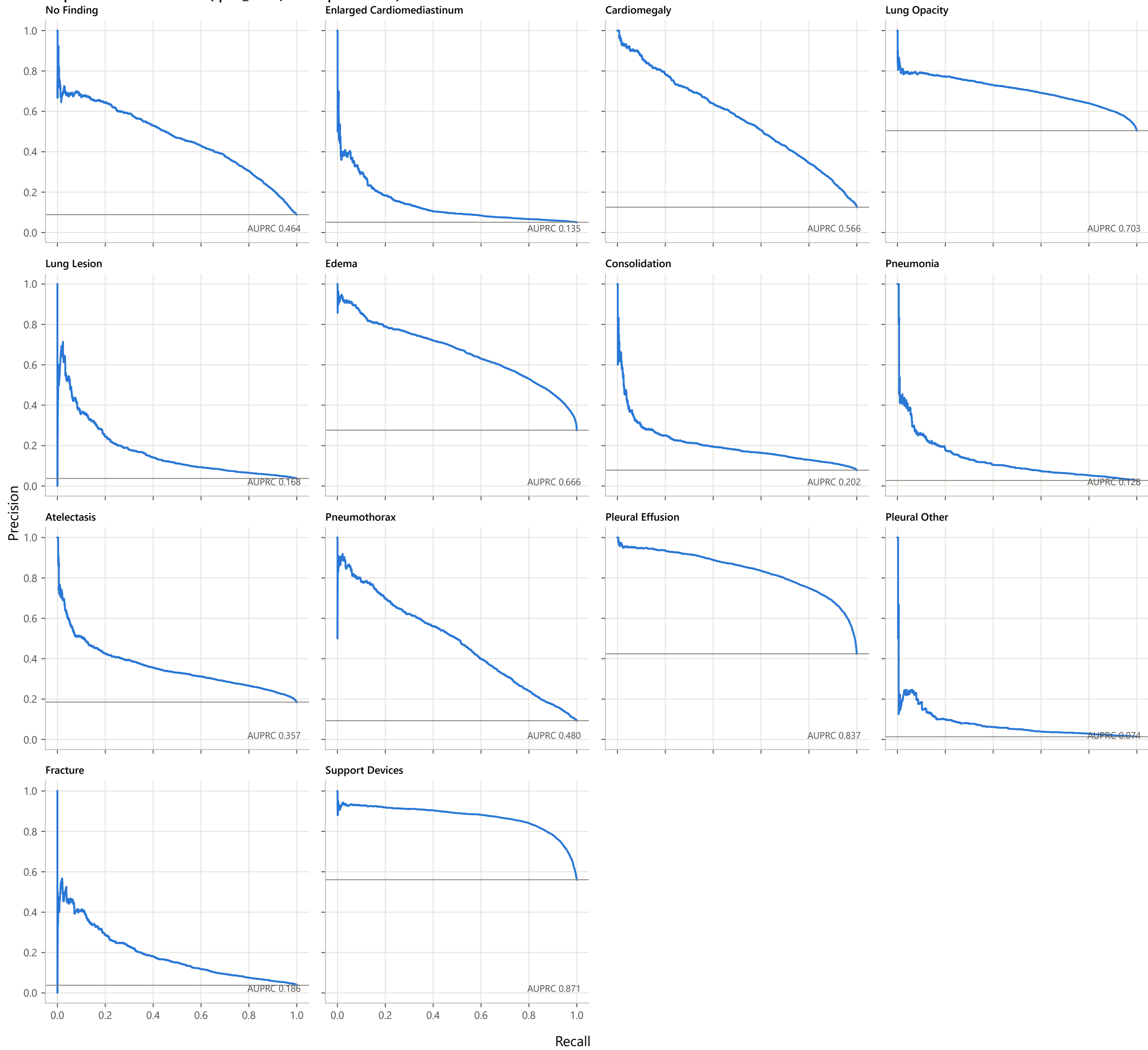
Validation precision-recall curves (fp32_strict; line = prevalence)
