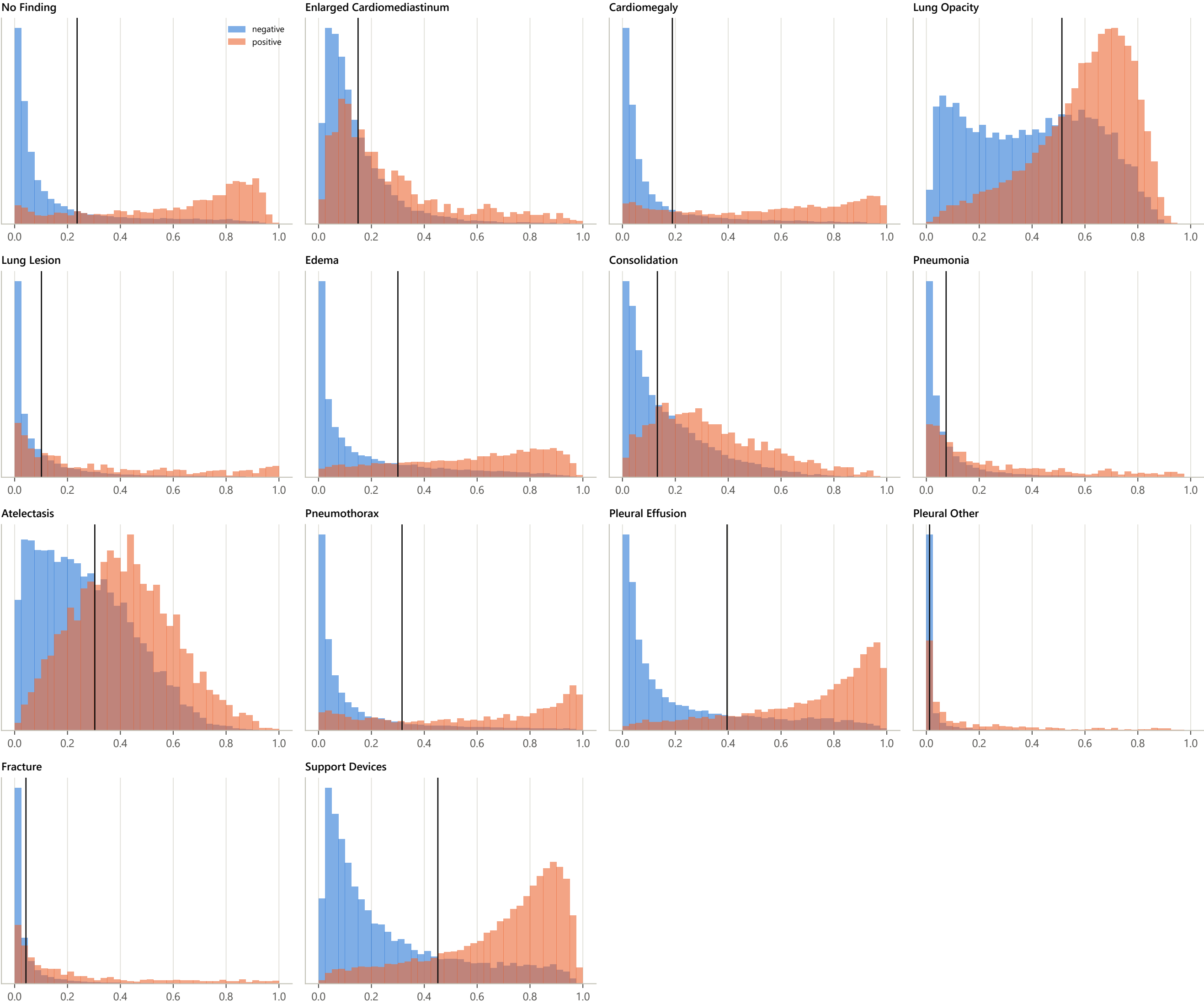
Validation probability distributions by true label (fp32_strict; line = Youden threshold)
