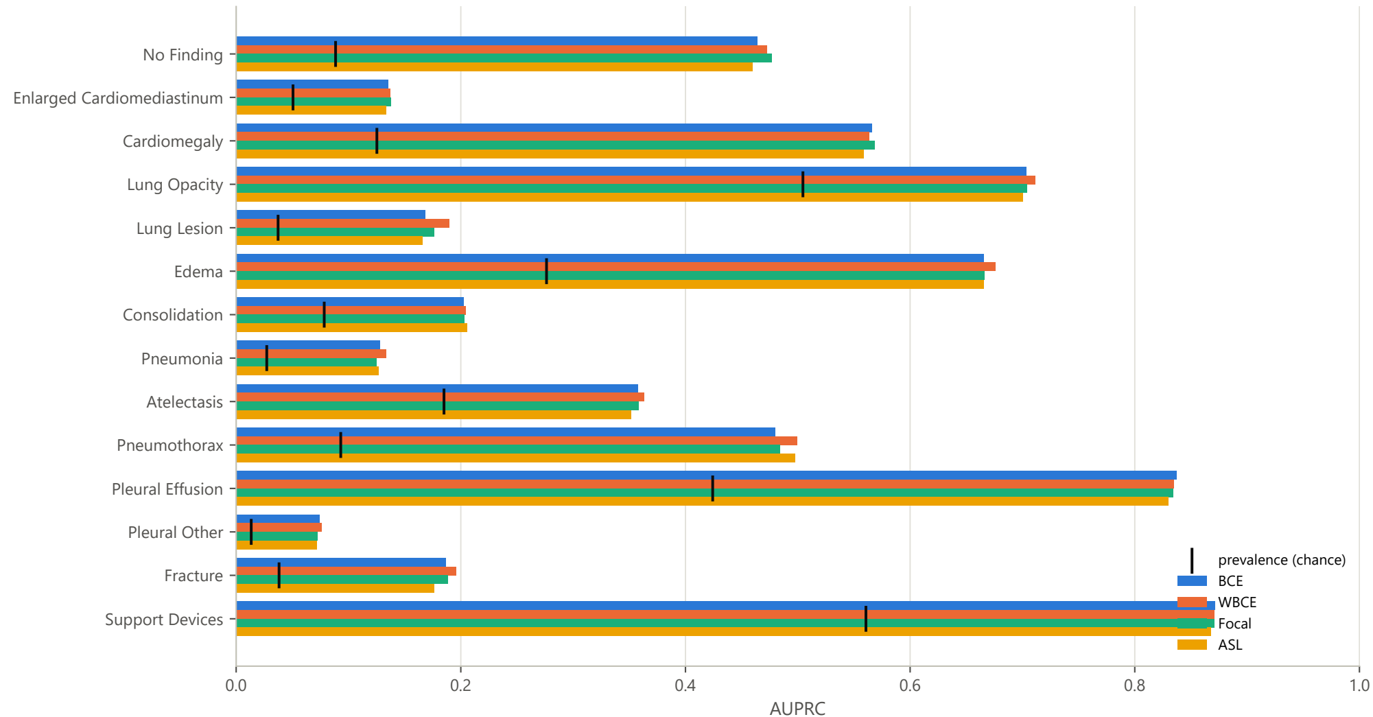
Per-class validation AUPRC by loss (all 14 classes)
