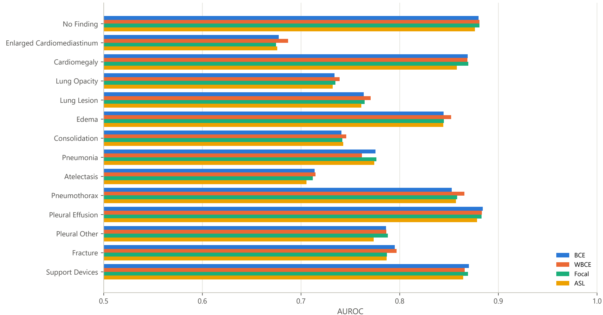
Per-class validation AUROC by loss (all 14 classes)
