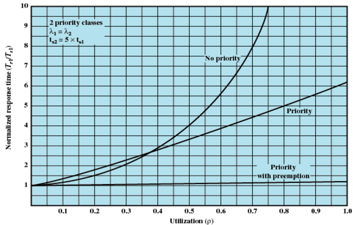
Figure 9.12 Normalized Response Time for Shorter Processes
