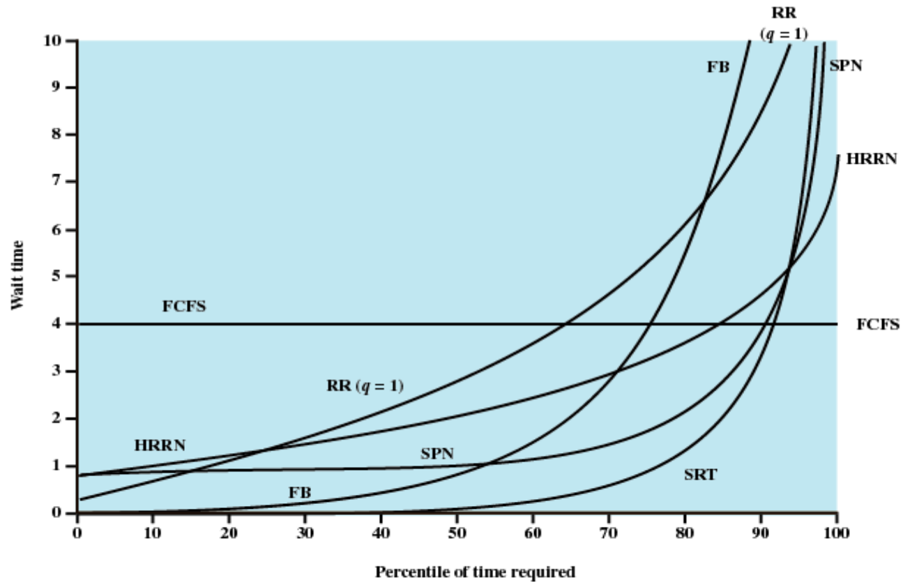
Figure 9.15 Simulation Results for Waiting Time
