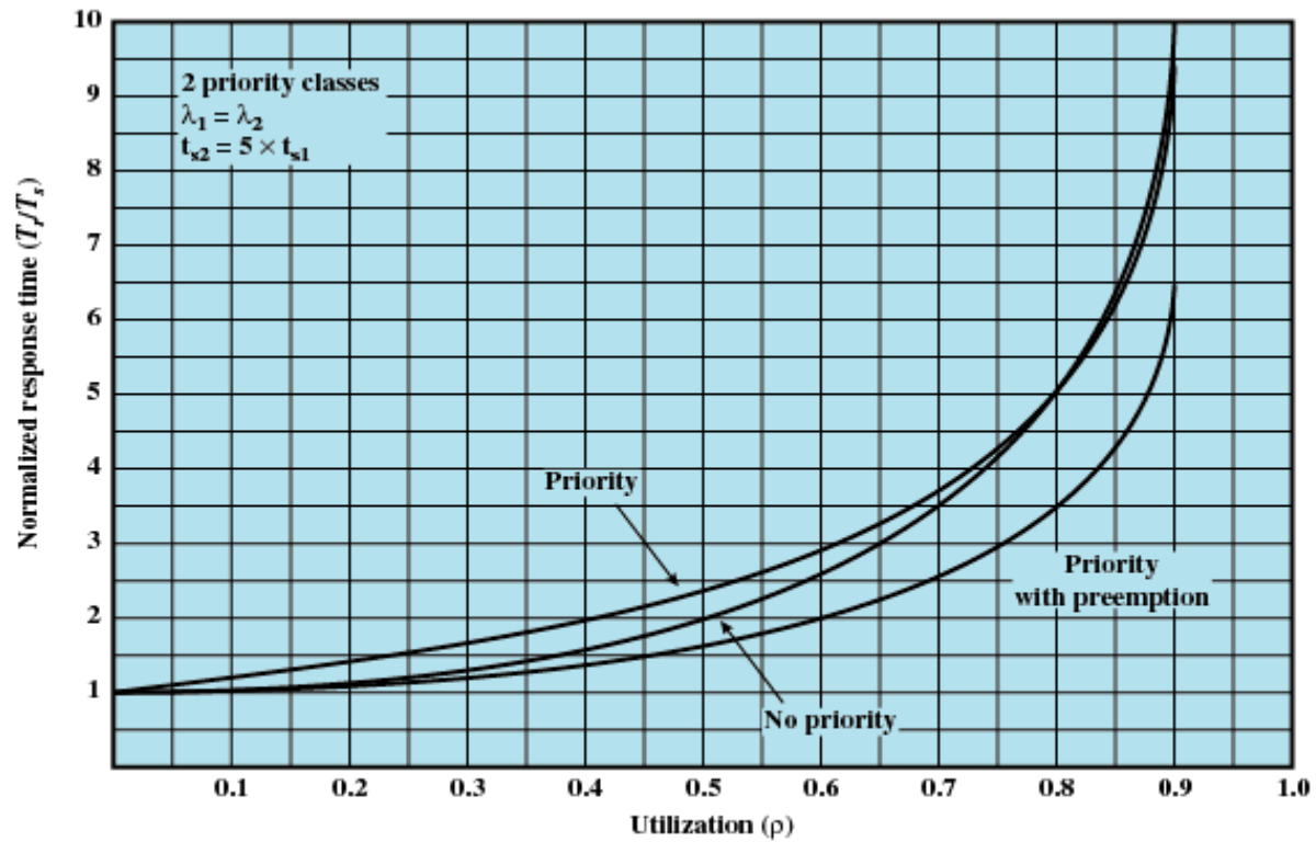
Figure 9.11 Overall Normalized Response Time
