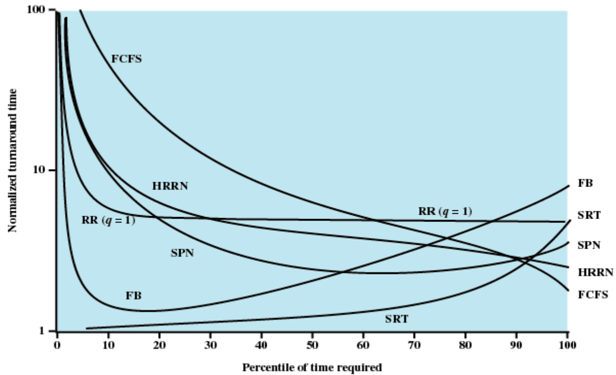
Figure 9.14 Simulation Results for Normalized Turnaround Time
