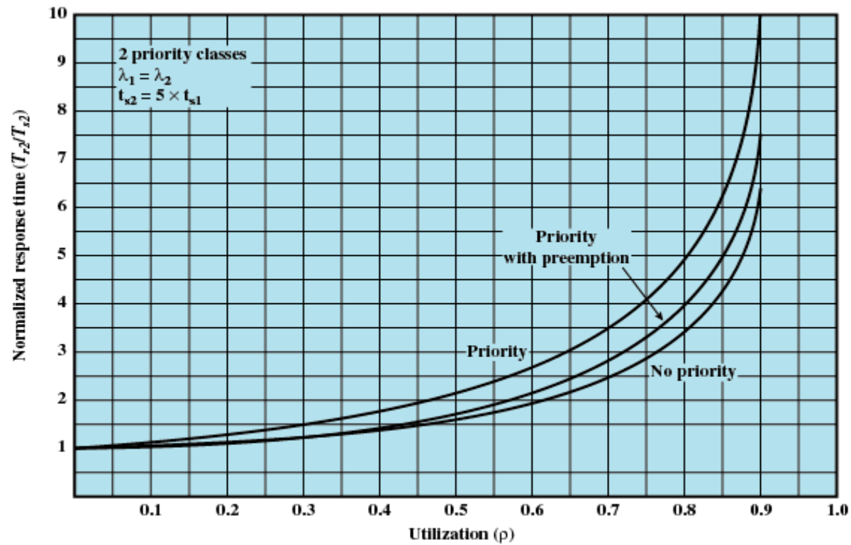
Figure 9.13 Normalized Response Time for Longer Processes
