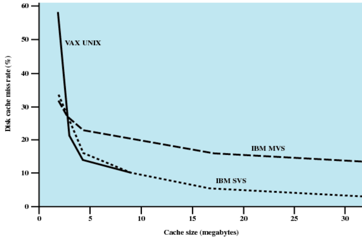
Figure 11.10 Some Disk Cache Performance Results Using LRU
