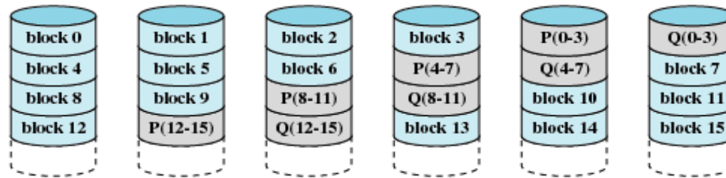
(g) RAID 6 (dual redundancy)
