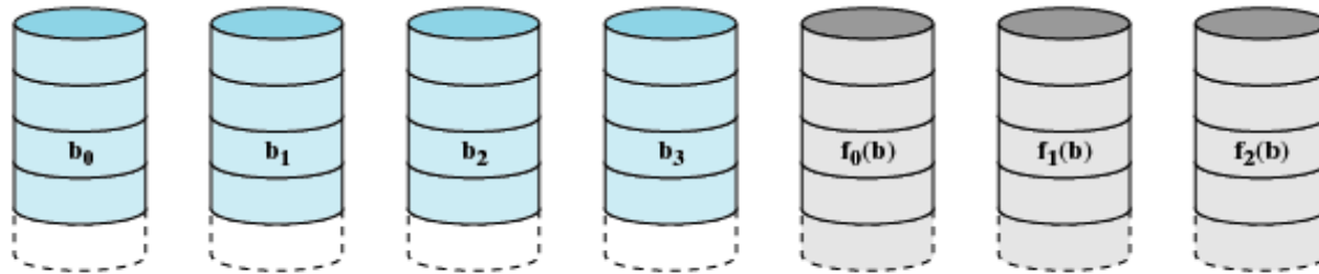
(c) RAID 2 (redundancy through Hamming code)
