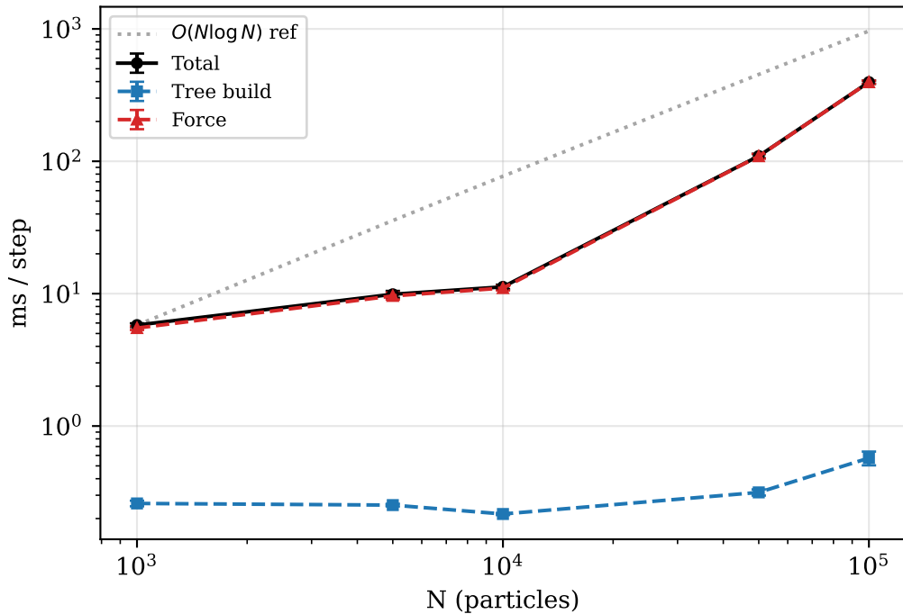
Plummer Sphere: Step Time vs Particle Count
