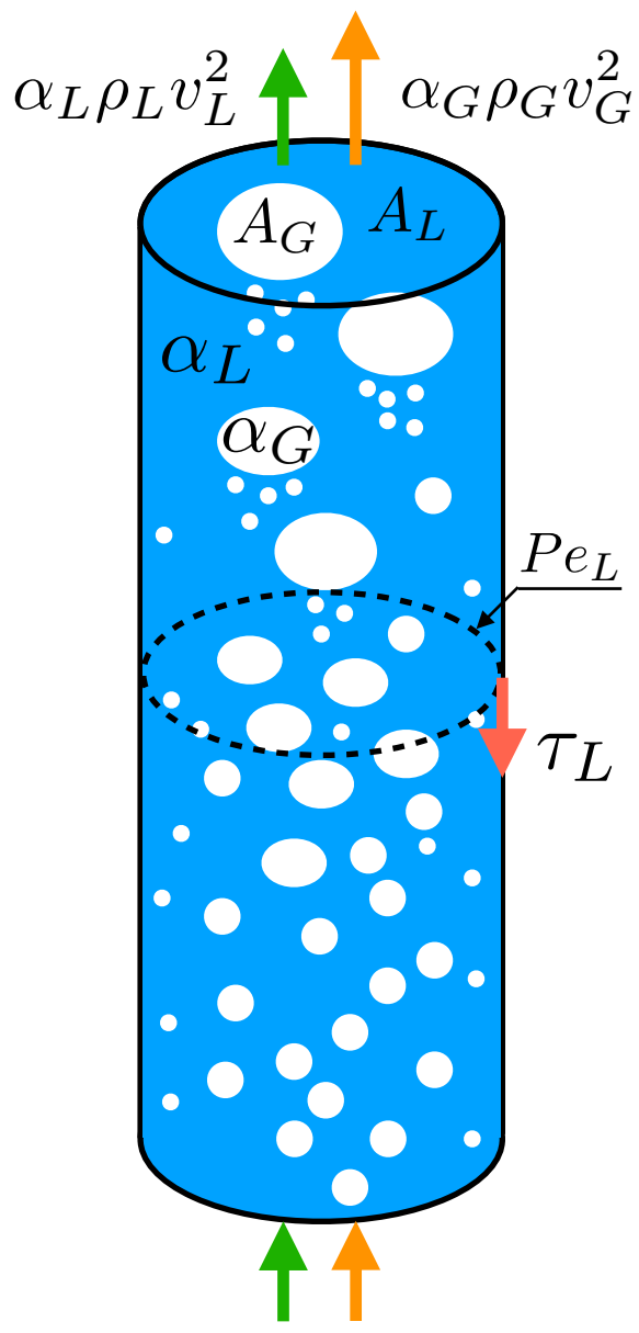
(a) upward flow in vertical pipe
