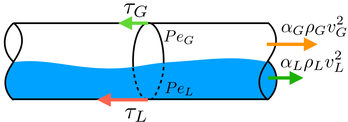
(b) horizontal pipe flow
