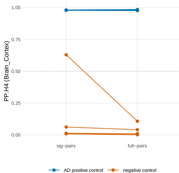
B Pre-specified panel (locus-signal subset)
