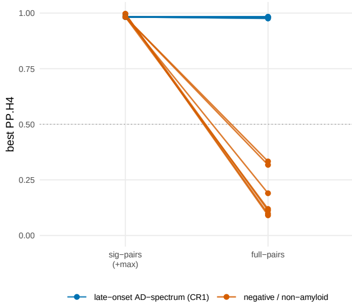
A Coloc-tested screening hits
