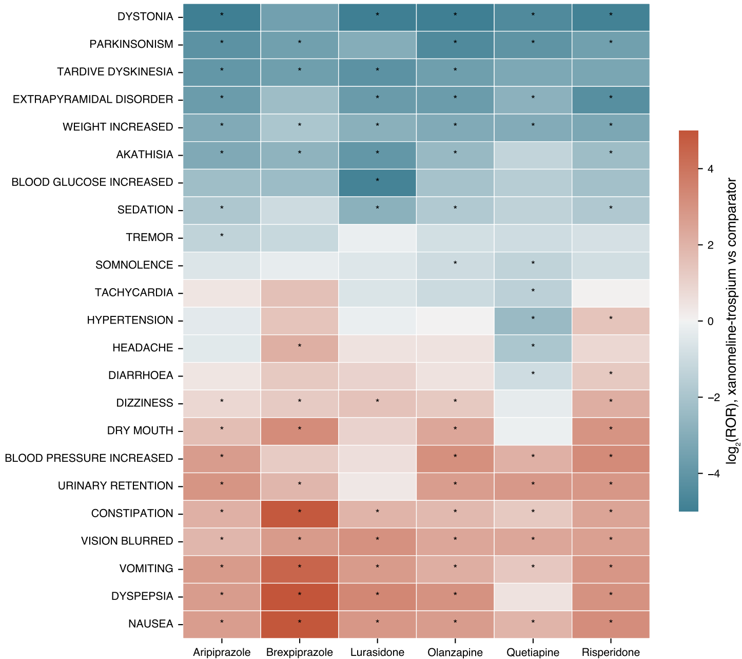
Active-Comparator Disproportionality: Xanomeline-Trospium vs D2 Antagonists (* = Bonferroni-significant)
