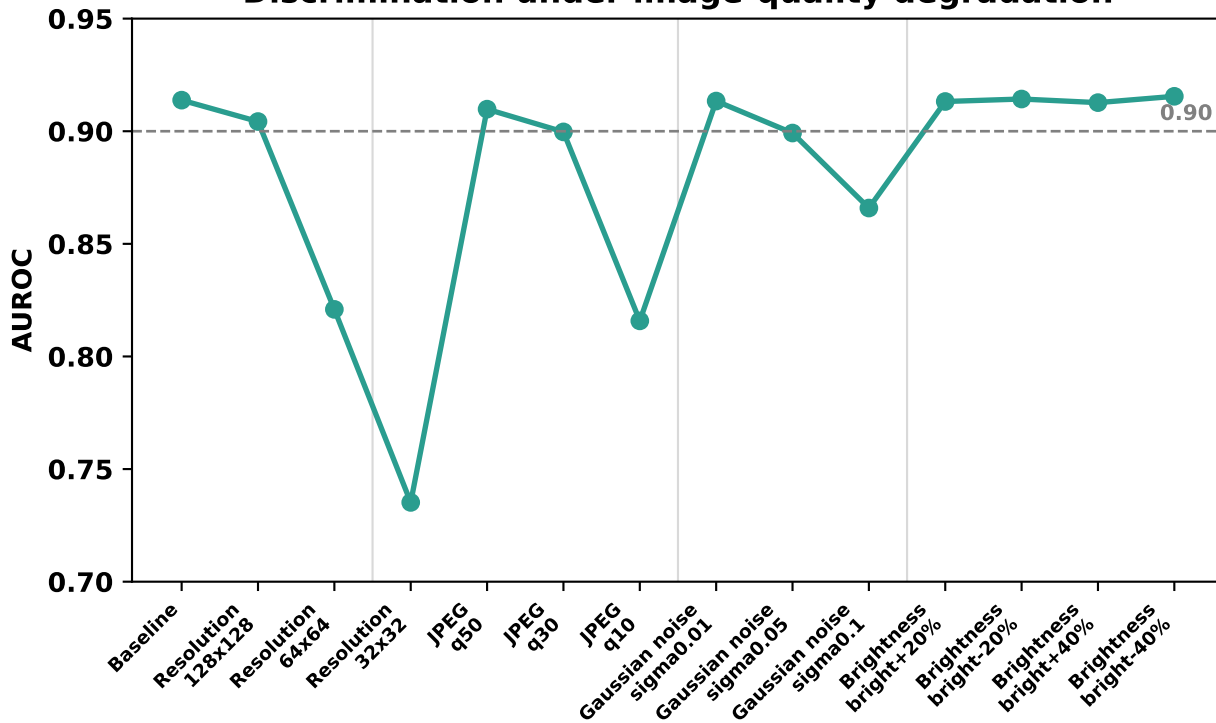
Discrimination under image-quality degradation
