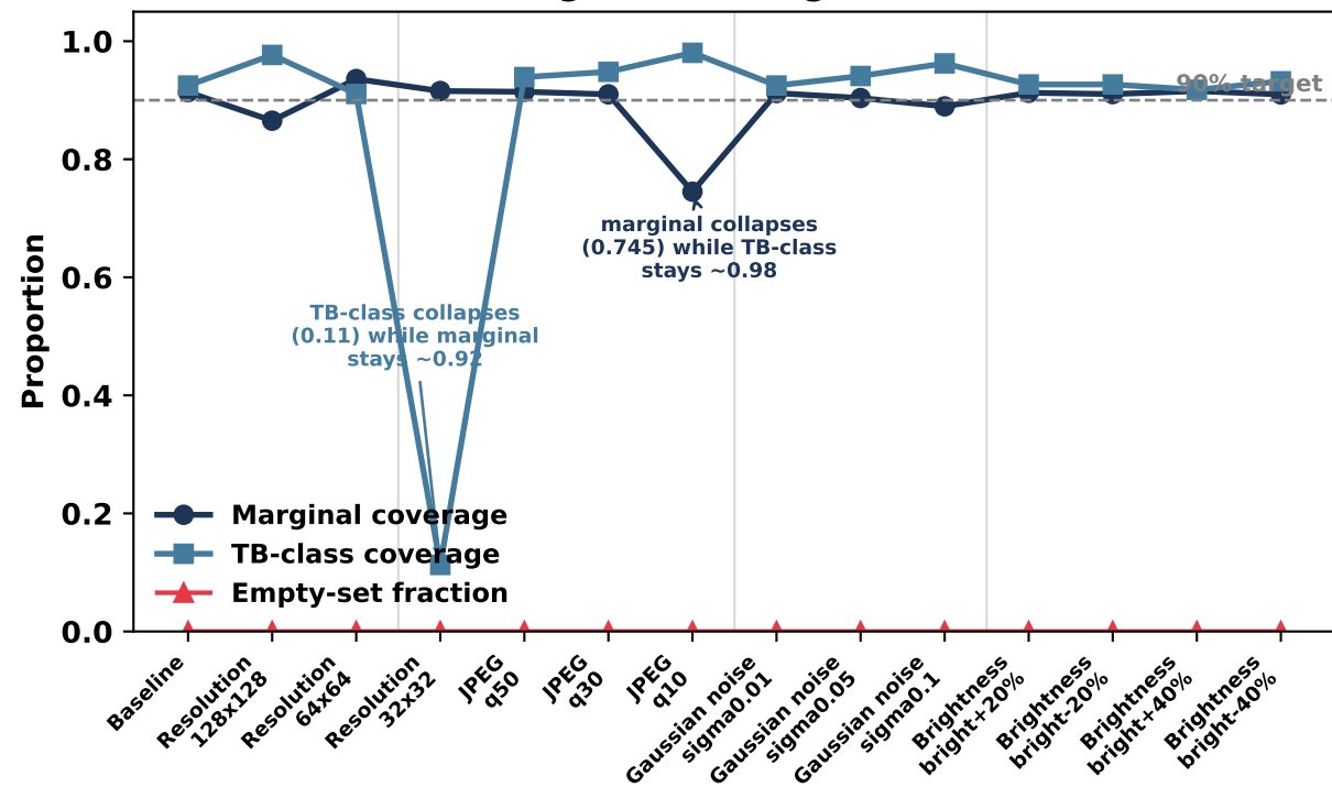
Coverage decoupling under degradation (TB-class can diverge from marginal in either direction)
