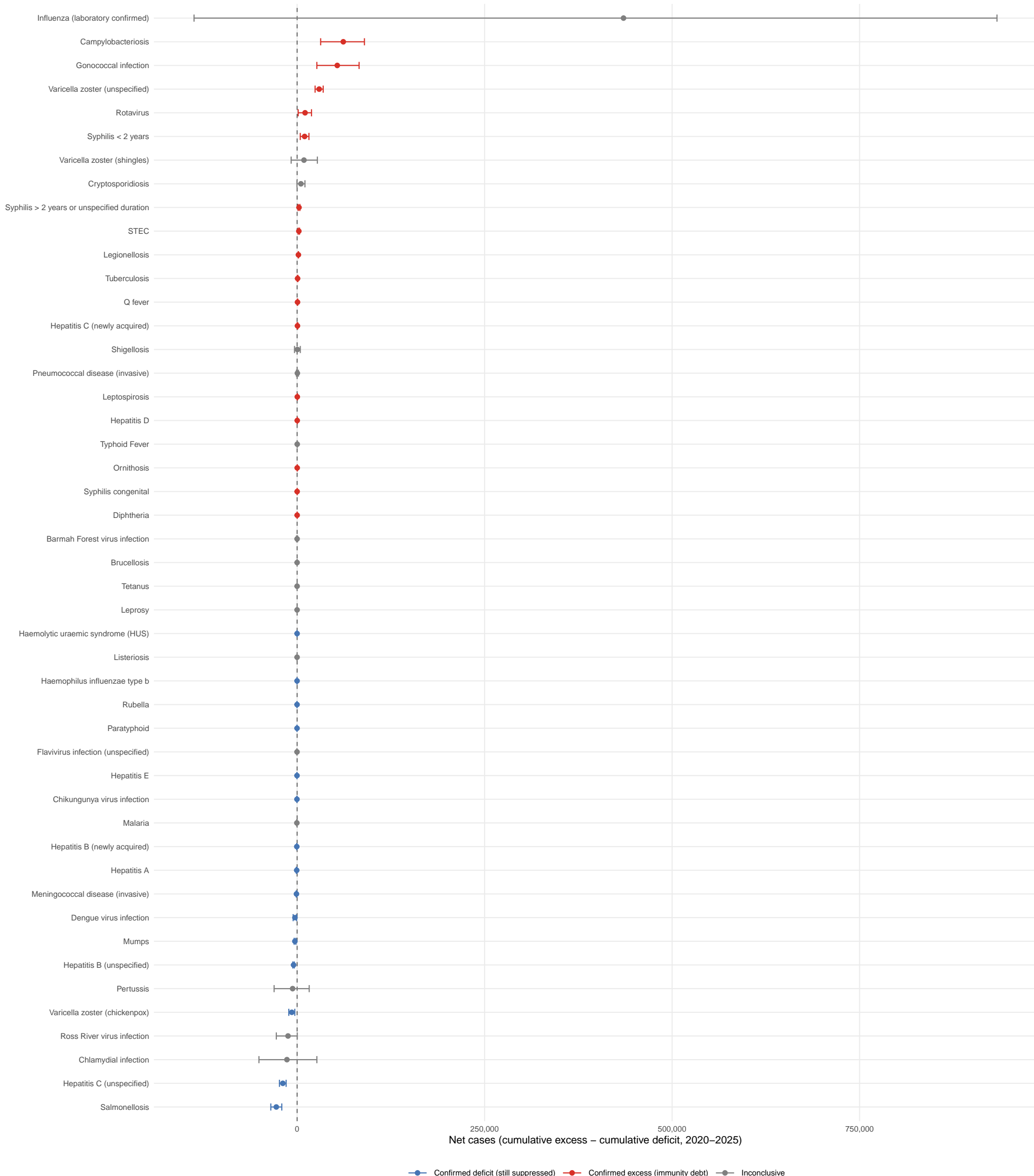
Figure 12. Cumulative Net Immunity Debt with 95% Bootstrap CIs
