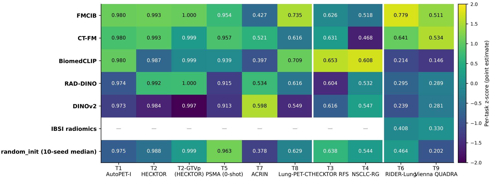
Figure 1. Cross-FM × cross-task primary-metric matrix. Cells annotated with point estimate; colour = per-task z-score.
