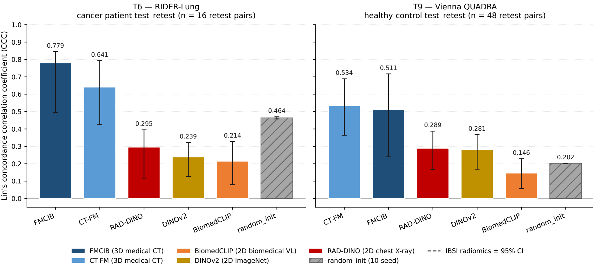
Figure 3. H6 — test-retest reproducibility on cancer (T6) and healthy controls (T9). FMCIB and CT-FM exceed IBSI; three FMs sit below.
