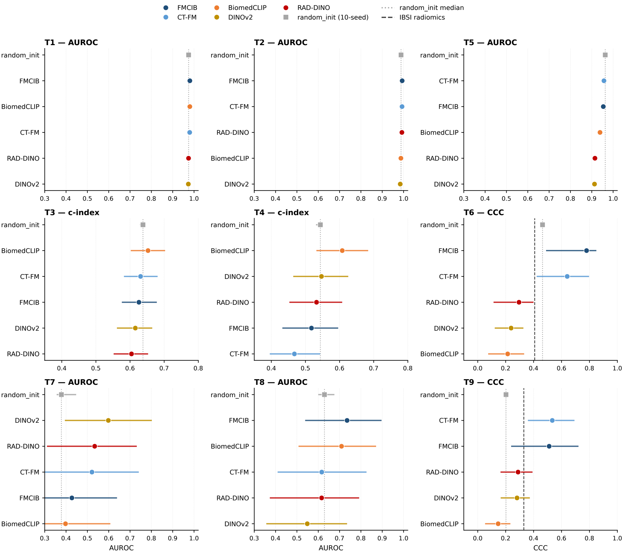
Figure 4. Per-task FM ranking with patient-clustered bootstrap 95% CI. Reference lines: random_init 10-seed median (dotted); IBSI baseline (dashed, T6/T9 only).
