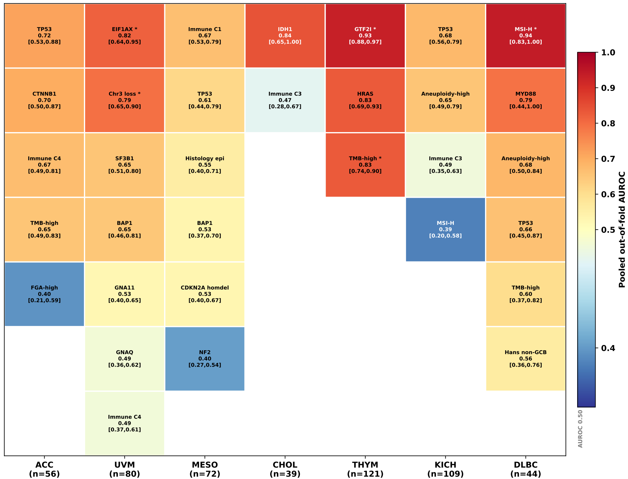
UNI2-h linear-probe AUROC across rare TCGA cohorts × biomarkers * = BH-FDR significant ( \alpha=0.05 ); bold = primary cell
