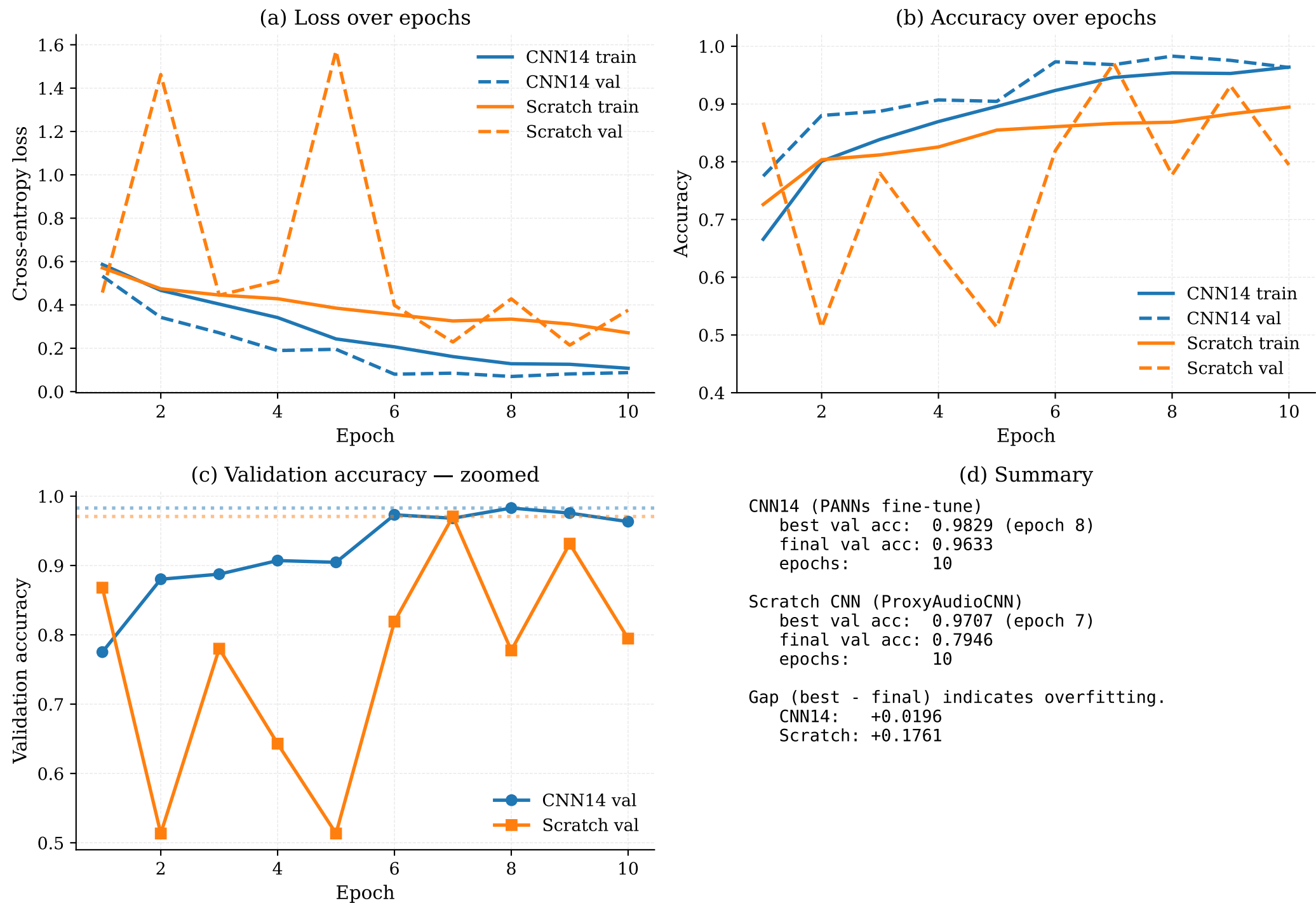
Figure 1 — Training dynamics: CNN14 (PANNs) vs scratch CNN
