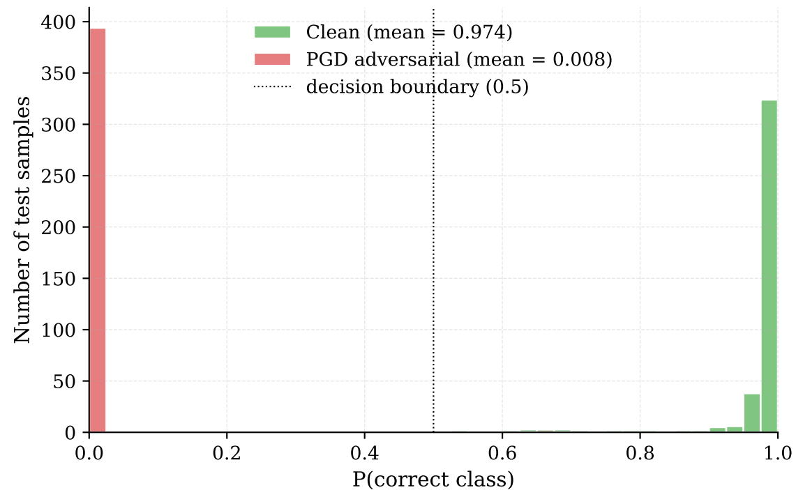
(a) Confidence distribution — \varepsilon = 0.001
