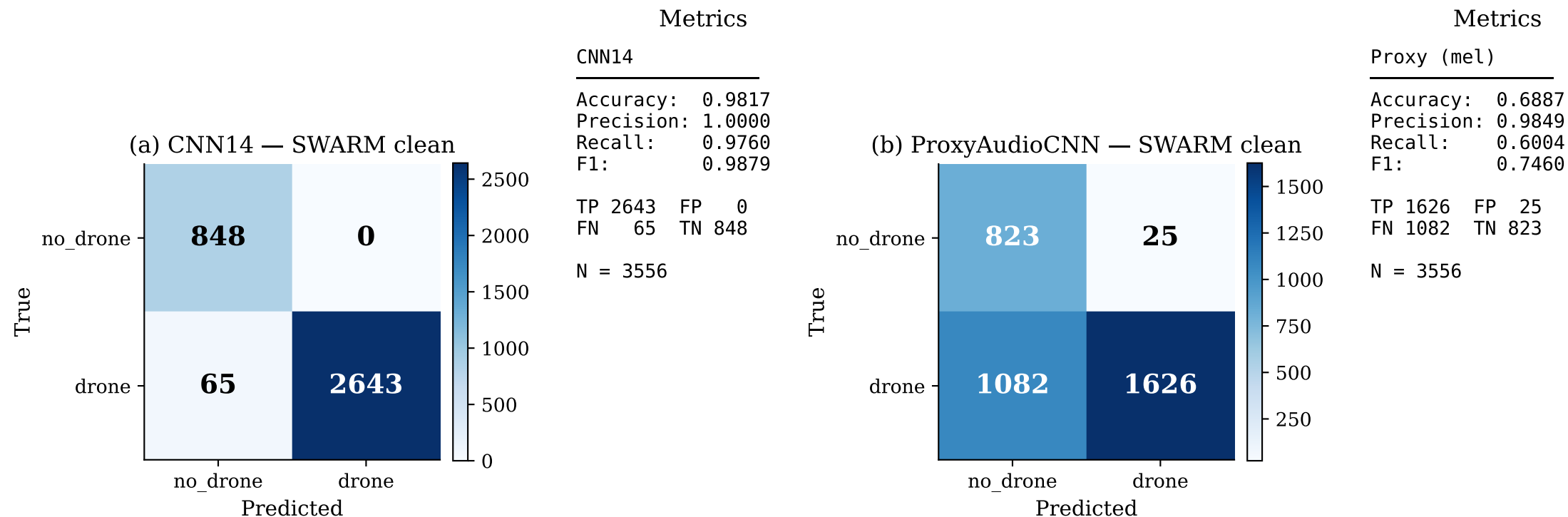
Figure 2 (cross-dataset) — Clean accuracy on SWARM (N = 3556)
