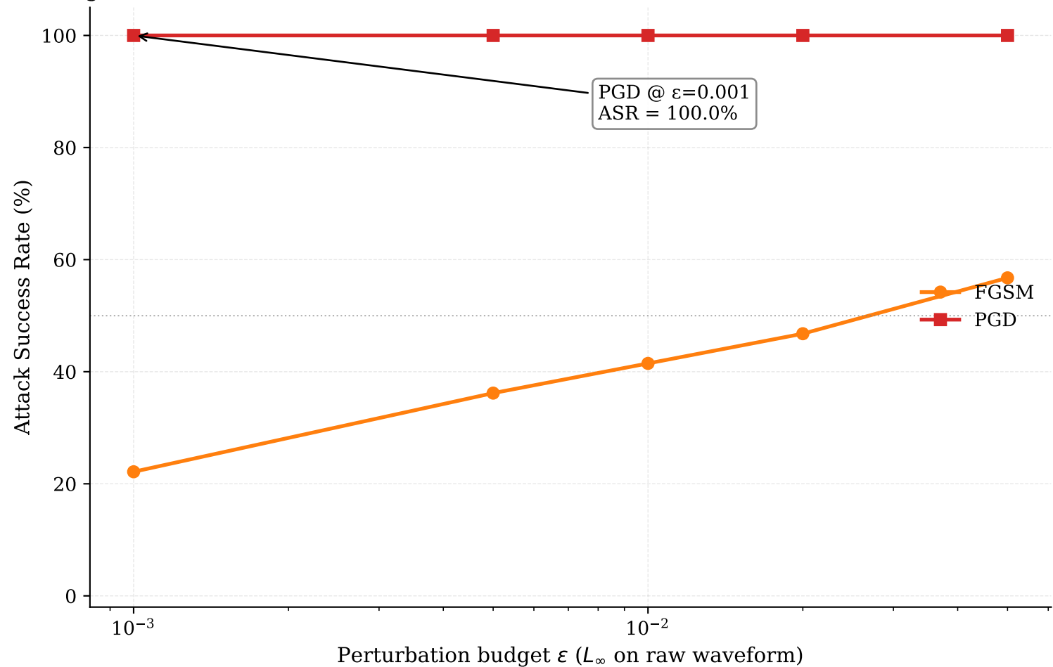
Figure 3 (cross-dataset) — ASR vs \varepsilon on SWARM (conditional, clean-correct denominator)
