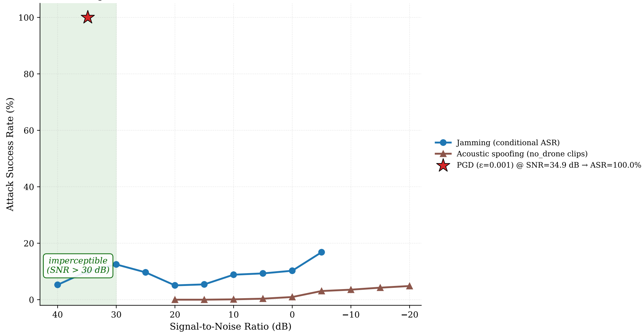
Figure 5 (cross-dataset) — Baselines vs PGD on SWARM
