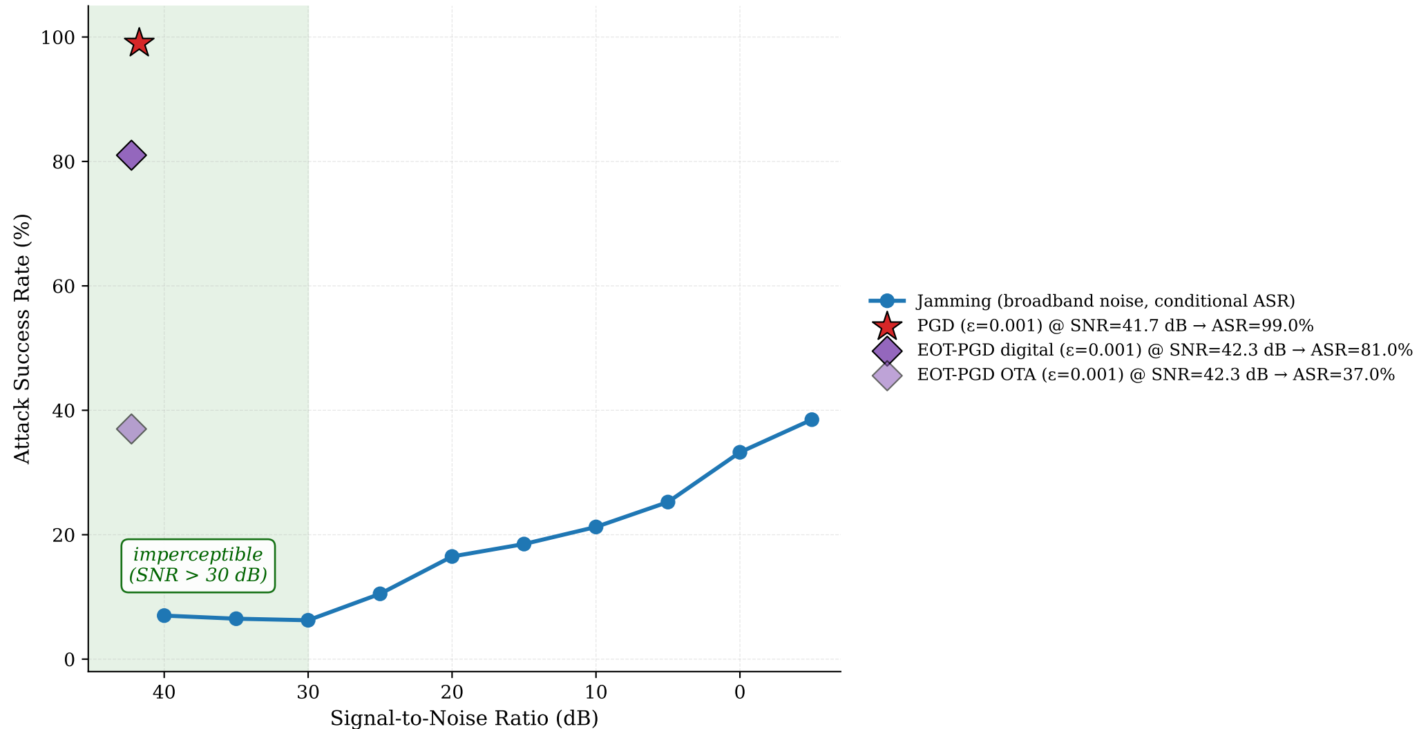
Figure 5 — Attack efficiency: gradient-based attacks vs jamming
