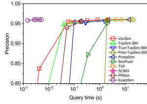
(a) Email-Eu-core
