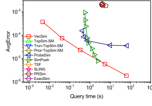
(c) Friendster
