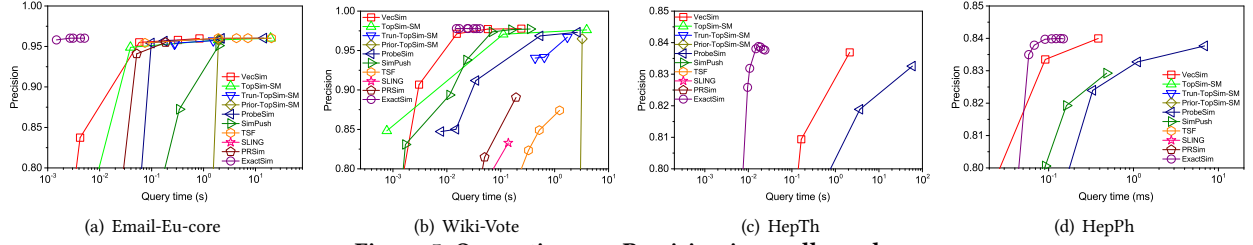
Figure 5: Query time v.s. Precision in small graphs
