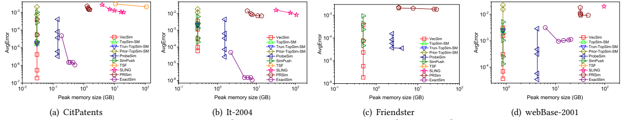
Figure 8: Peak memory v.s. AvgError v.s. in large graphs
