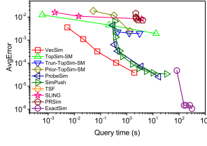
(b) It-2004
