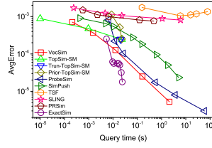
(c) HepTh
