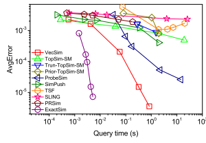
(a) Email-Eu-core
