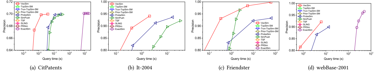
Figure 7: Query time v.s. Precision in large graphs
