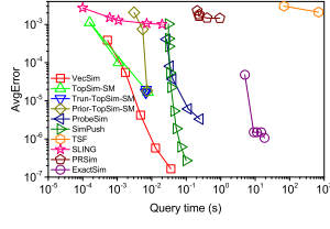
(a) CitPatents
