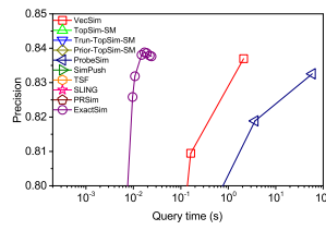
(c) HepTh
