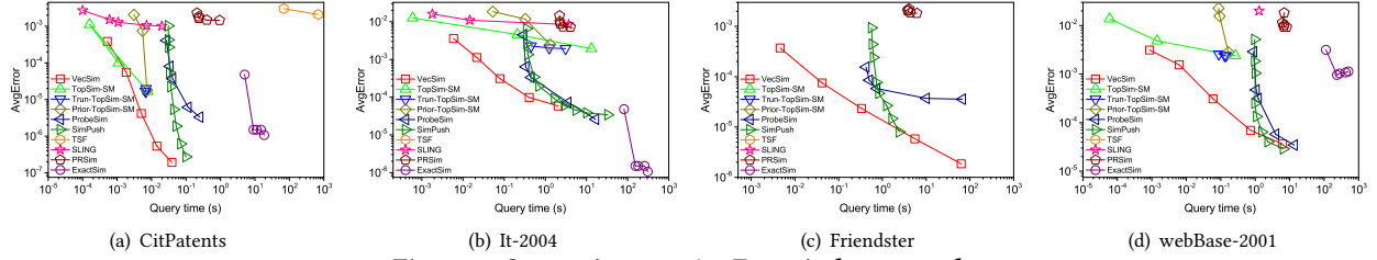
Figure 6: Query time v.s. AvgError in large graphs
