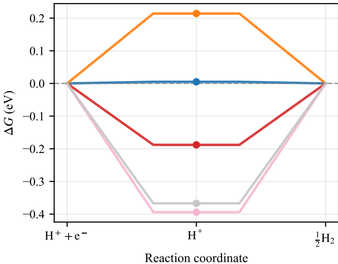
HER Gibbs Free Energy Diagram
