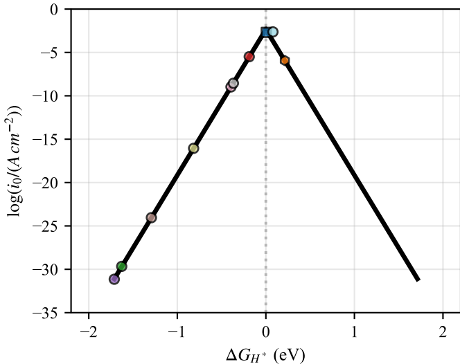
Volcano Plot for 2D W-N materials
