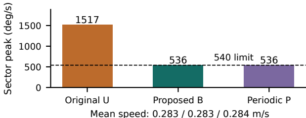
(b) Measured at a 0.45 m/s command
