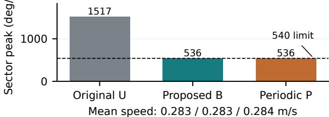
(b) Measured at 0.45 m/s command
